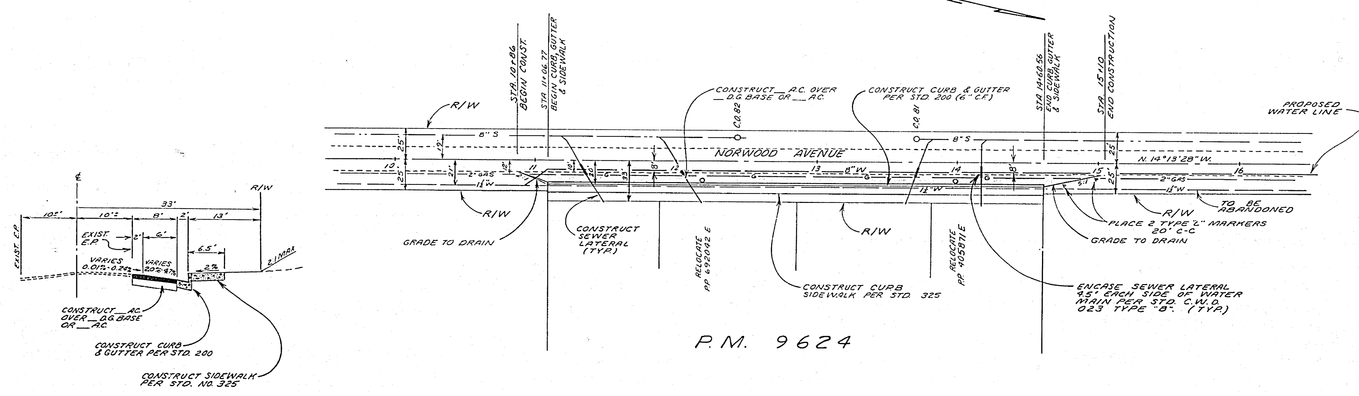
NORWOOD AVE T.I. - 6 TYPICAL SECTION NO SCALE
