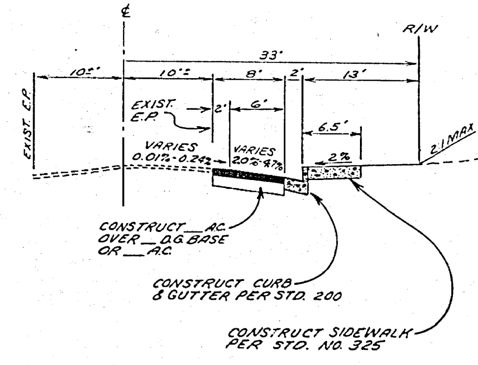
NORWOOD AVE T.I. - 6 TYPICAL SECTION NO SCALE
