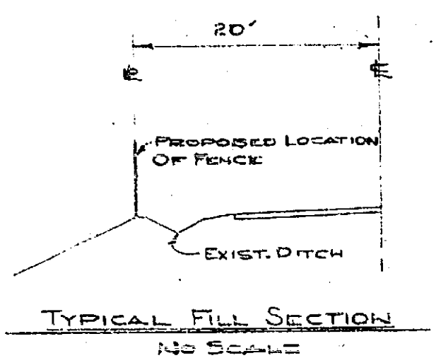
TYPICAL FILL SECTION NO SCALE FENCE TO BE ON R.O. OR IN A STRAIGHT LINE ON SLOPE, AS DIRECTED BY ENGINEERS.
