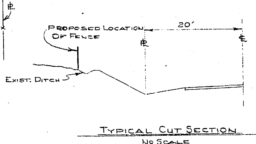
TYPICAL CUT SECTION NO SCALE FENCE TO FOLLOW TOP OF CUT.
