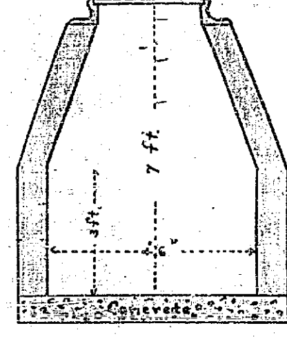
Cross Section of Flush Tank. Scale 3ft. = 1in.
