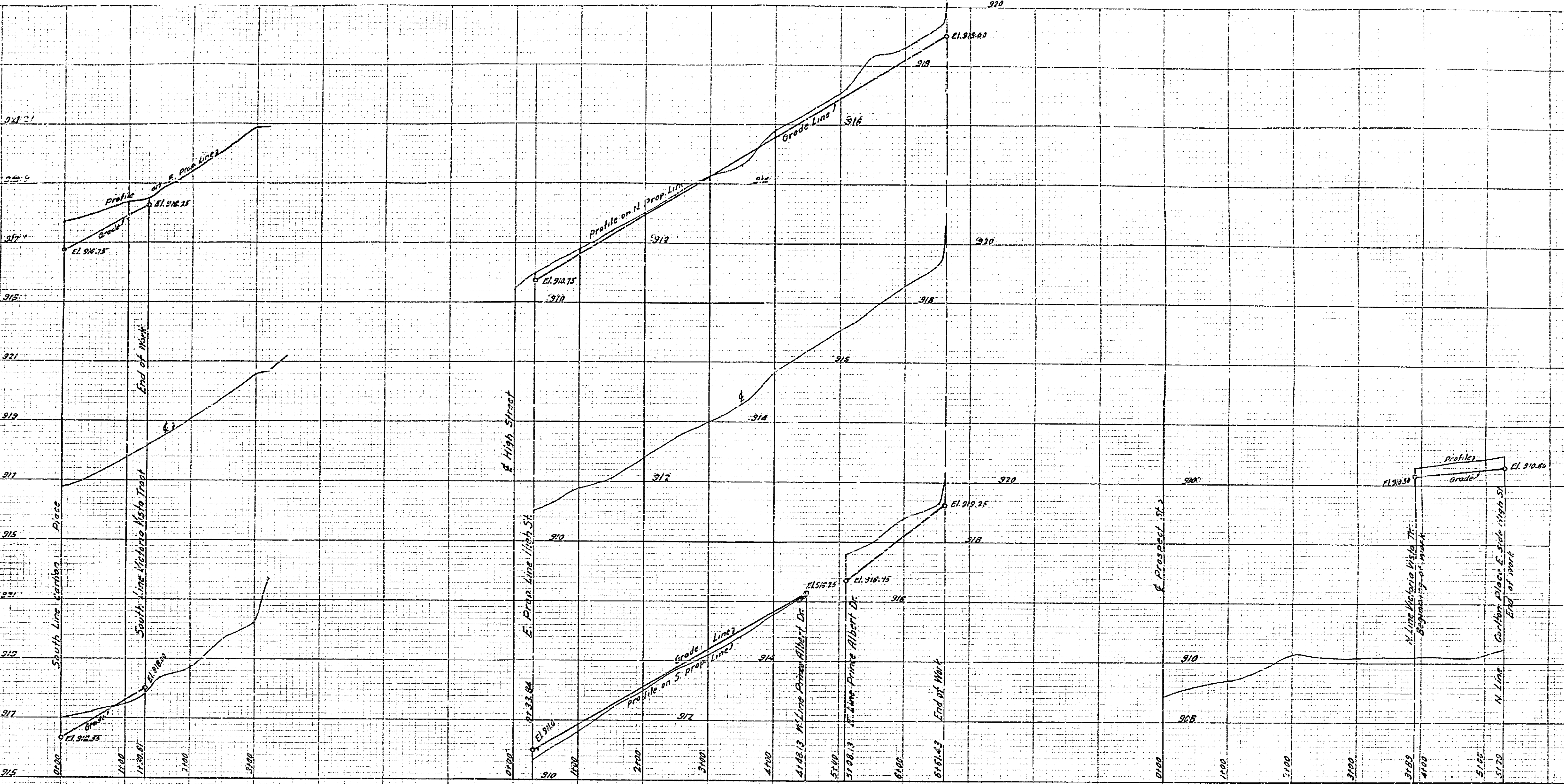
PROFILES OF VICTORIA VISTA TR. SCALES { HORIZ. 1"=100' VERT. 1"=2'
