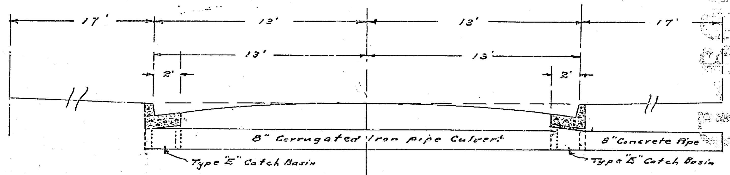
Cross-Section showing Catch Basins & Culvert.
