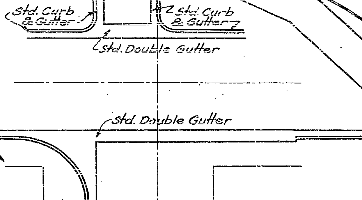
TYPICAL INTERSECTION Scale 1"=20'
