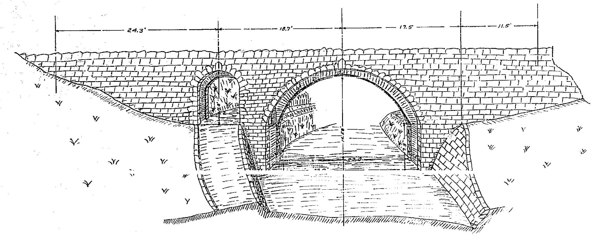
DETAIL OF BUENA VISTA AVE. BRIDGE LOOKING NORTHWESTERLY TOPOGRAPHICAL MAP WESTERN ENTRANCE TO RIVERSIDE CITY. BUENA VISTA AVE., W. 8th ST., AND W. 7th ST. RIVERSIDE CITY PLANNING COMMISSION. MARCH 7, 1928.
