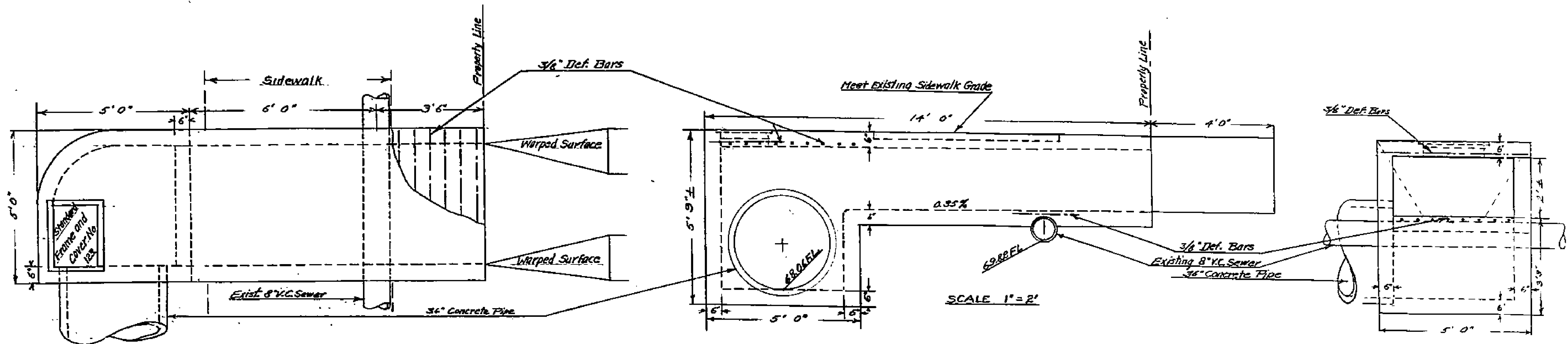
CONCRETE BOX INTAKE AND CATCH BASIN DETAILS.
