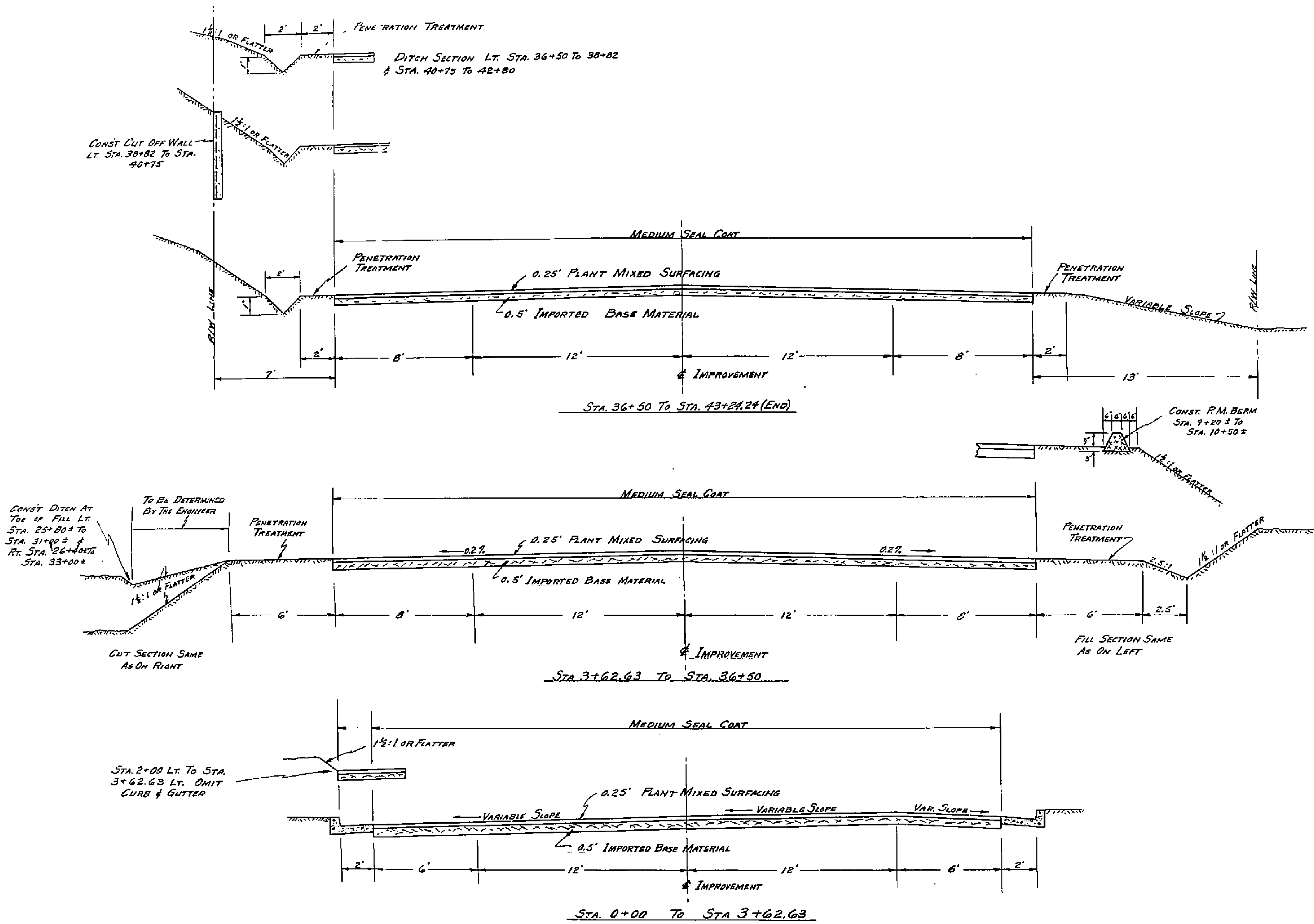
TYPICAL CROSS SECTIONS (SUPERELEVATION AS SHOWN ON PLANS AND AS DIRECTED BY ENGINEER) SCALE: 1"=3"
