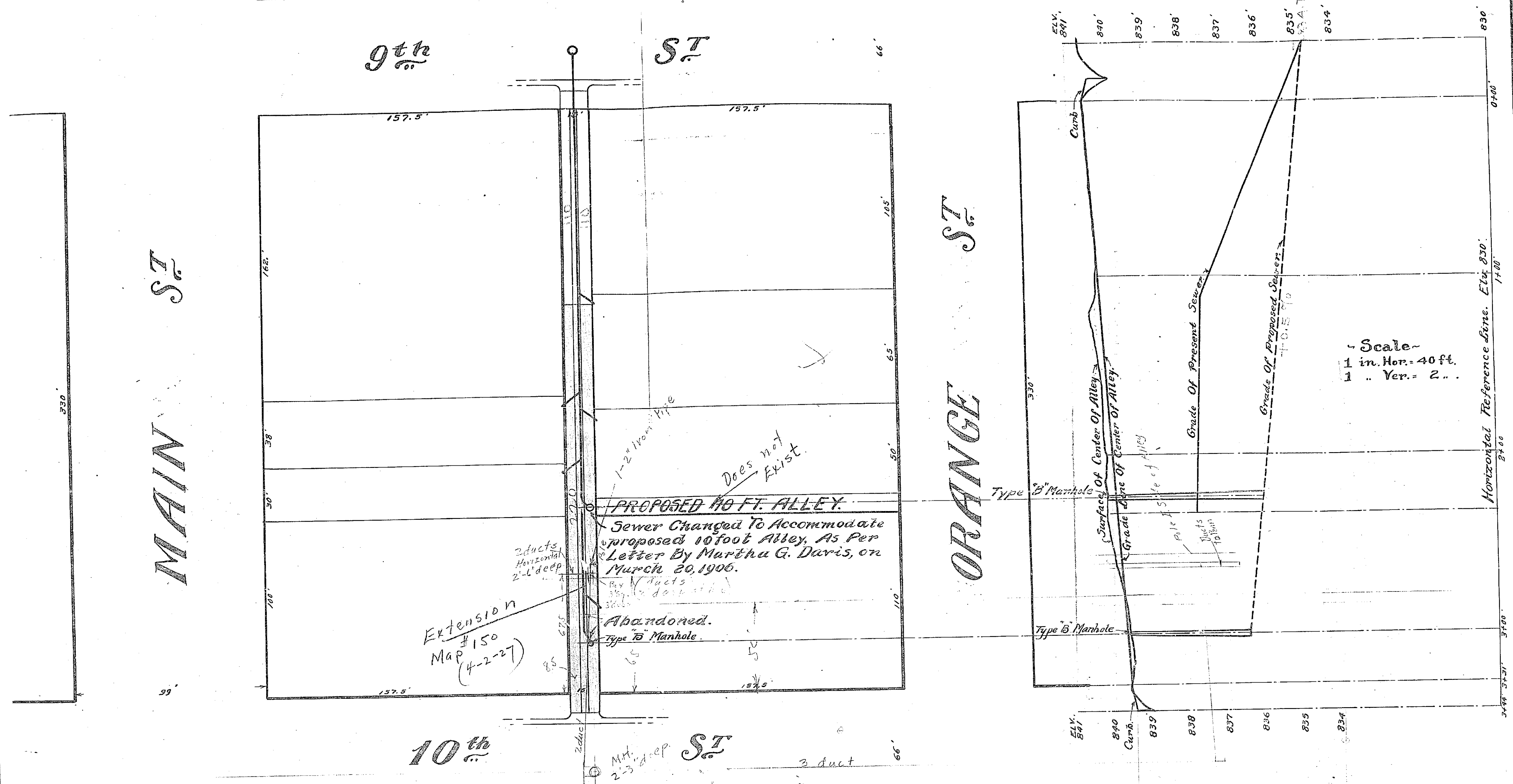
MAP of ALLEY In Block 9 Range 6 Showing Proposed Asphalt Pavement And Proposed Reconstruction of Sewer.
