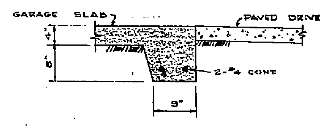
SECTION C SCALE 1\"/>
