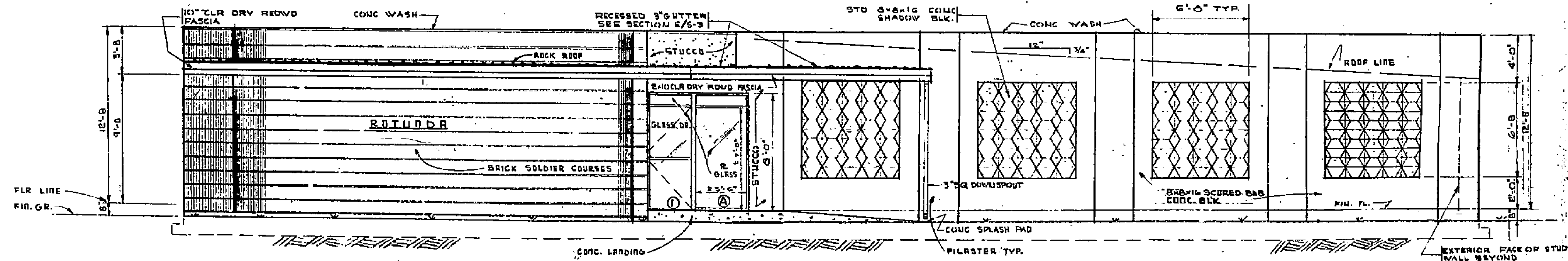
WEST ELEVATION SCALE: 1/4" = 1'-0"
