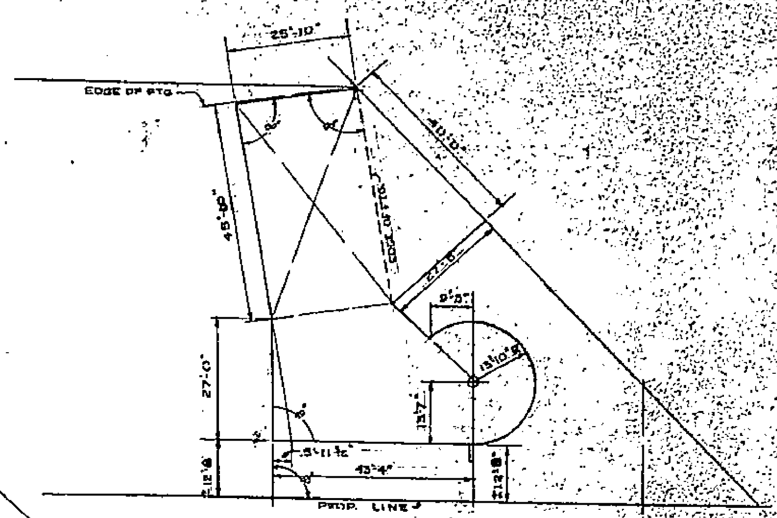
LAYOUT PLAN SCALE 1"=20'-0"
