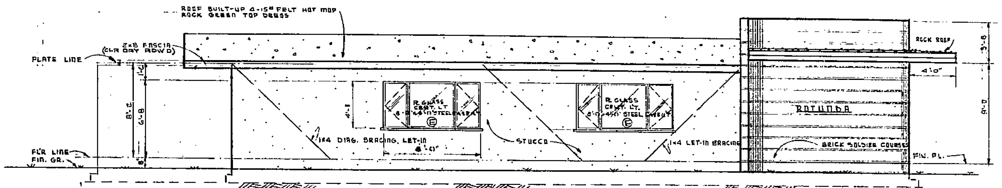
NORTH ELEVATION SCALE: 1/4" = 1'-0"
