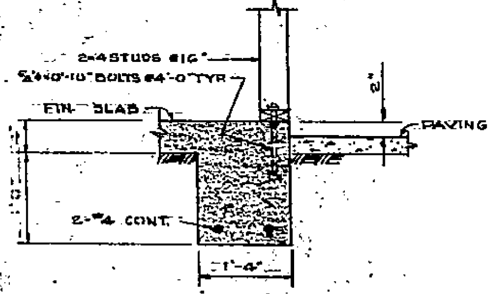
SECTION B SCALE 1\"/>
