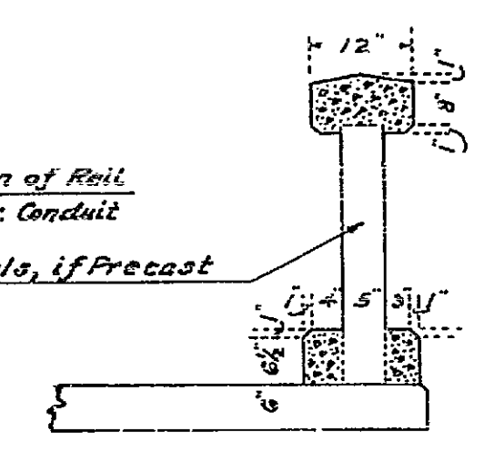
DETAIL SECTION OF RAILING Reinforcing not shown, Duplicate Existing Steel Reference Victoria Avenue Bridge Plans 1155
