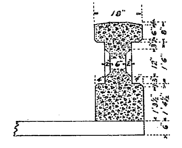
DETAIL SECTION OF RAILING Reinforcing not shown, Duplicate Existing Steel
