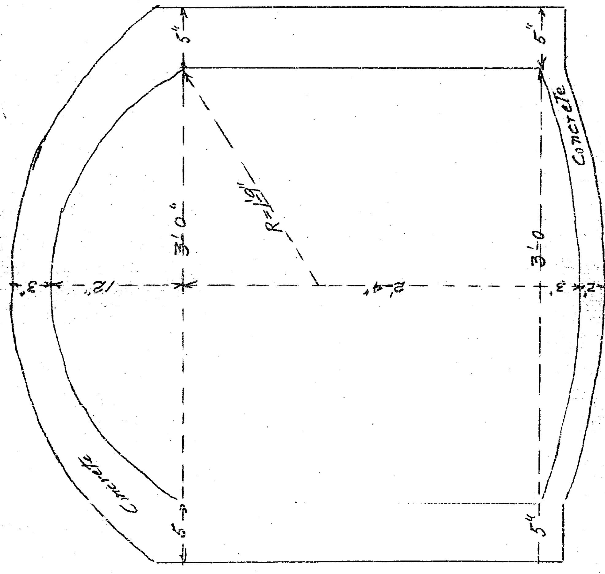
PLAN OF NORTH ORANGE ST CULVERT Scale 1/2" = 1'
