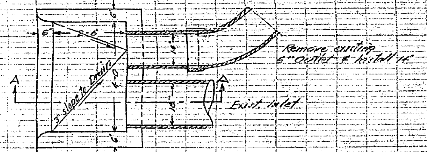
PLAN EXISTING CATCH BASIN Scale: 1 in. = 2 ft.
