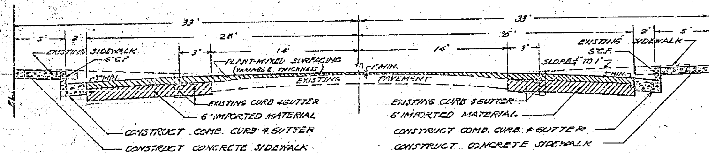
TYPICAL CROSS-SECTION
