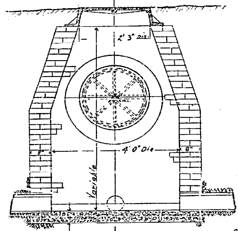
STANDARD Type "A" Manhole. For construction see Specifications No. 16.
