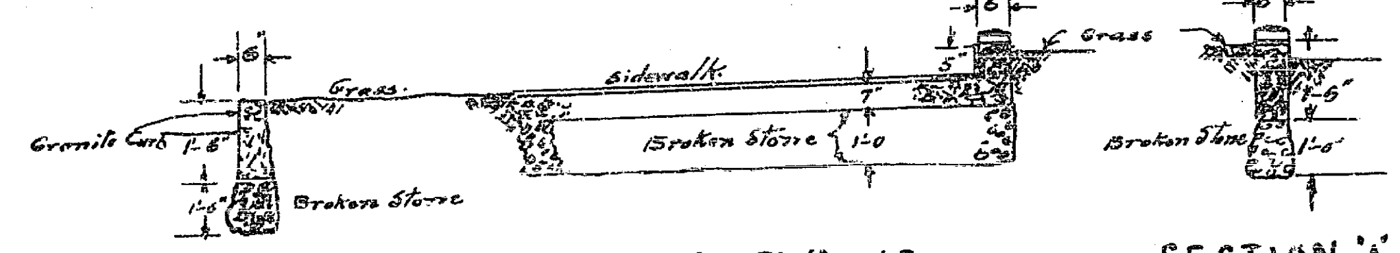
SECTION THRO SIDEWALKS SCALE 1/8" = 1'-0"
