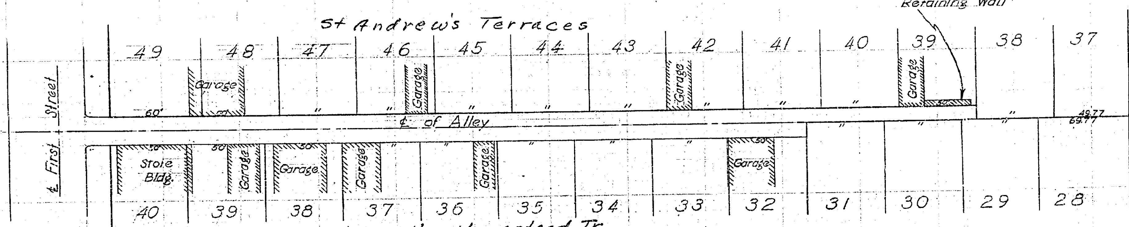
PLAN PROFILE OF ALLEY No. 689 Between Mulberry & Lime North of First
