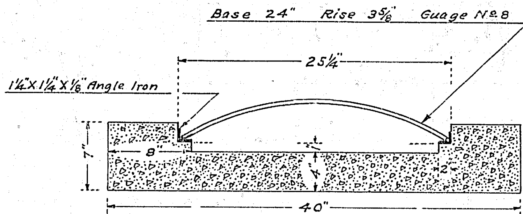
SECTION OF CULVERT Scale 1/2" = 1 Ft.
