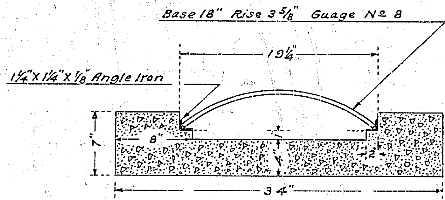
SECTION OF CULVERT Scale 1/2" = 1 Ft.
