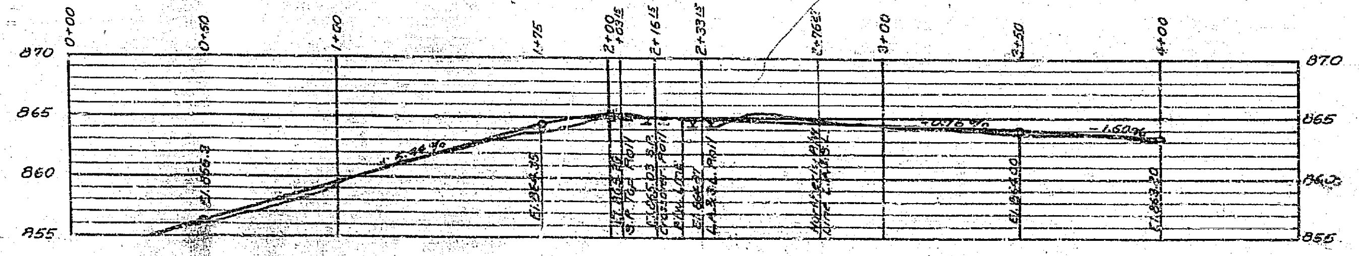
PROFILE OF NORTH MULBERRY ST. AT PROPOSED CROSSING
