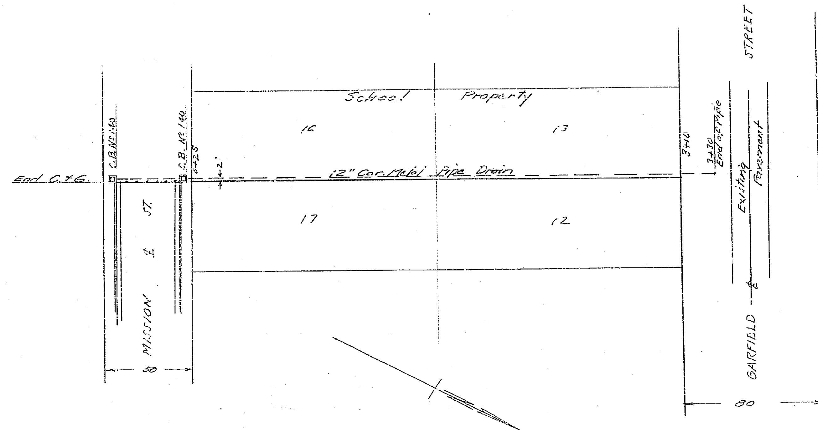
PLAN SCALE: 1 IN. = 40 FT.
