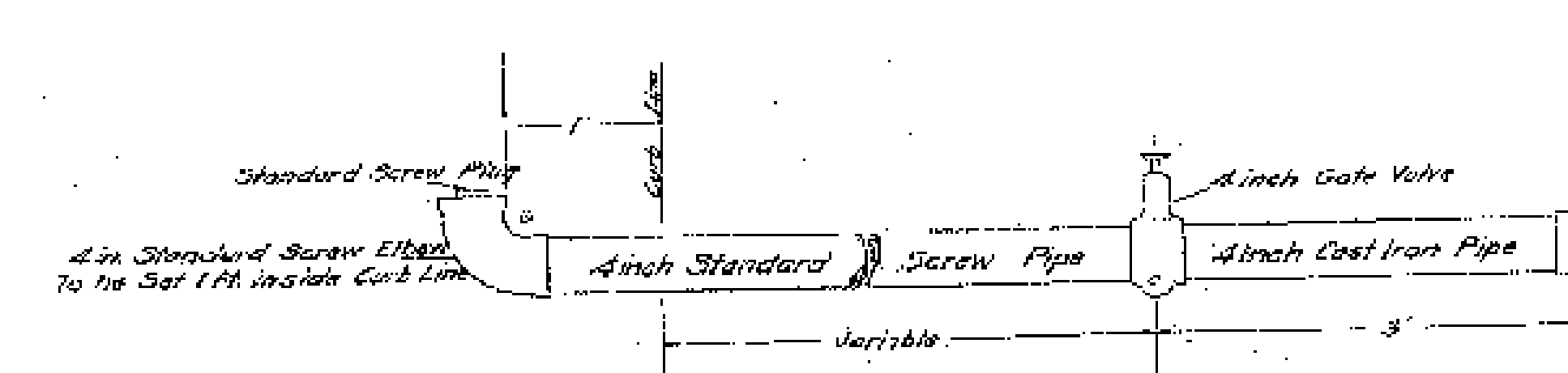
DETAIL OF 4 INCH OUTLET FOR FIRE HYDRANTS
