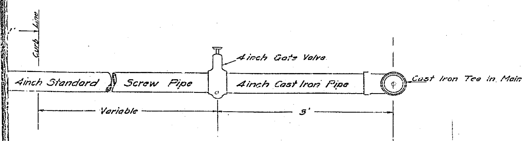
DETAIL OF 4 INCH OUTLET FOR FIRE HYDRANTS
