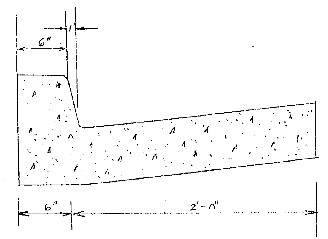
CURB & GUTTER DETAIL
