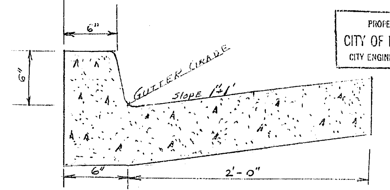
CURB & GUTTER DETAIL
