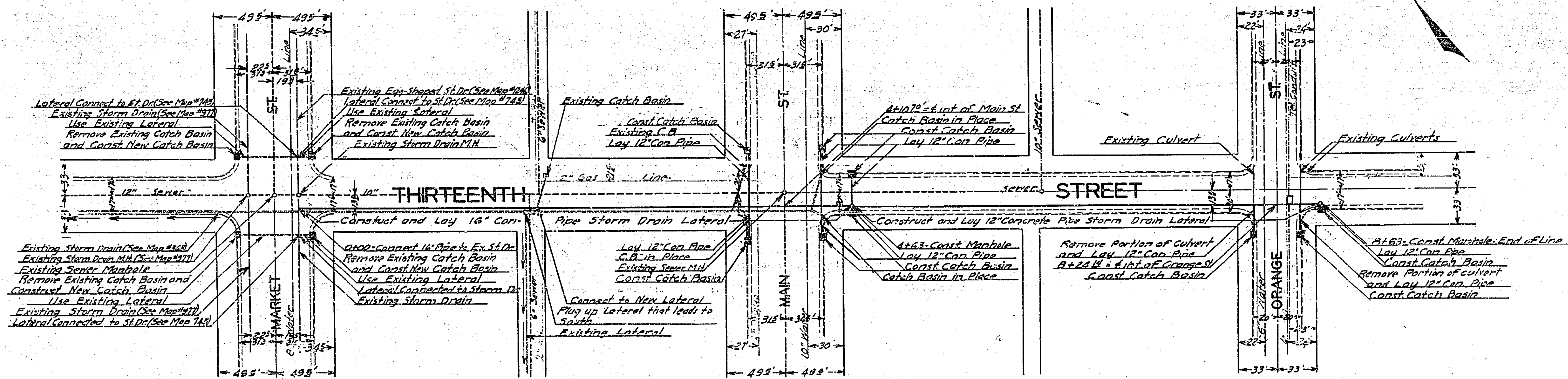
PLAN THIRTEENTH STREET SCALE 1" = 40'
