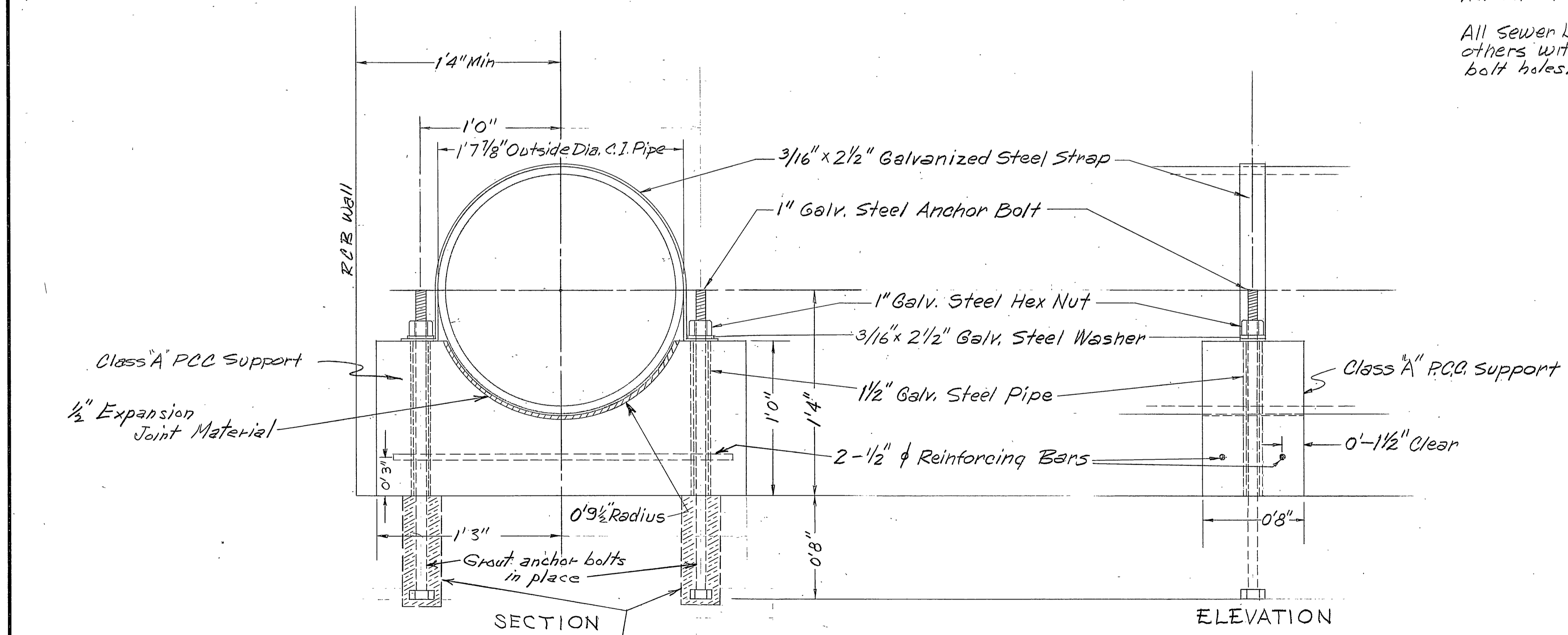
PIPE SUPPORT DETAIL No Scale
