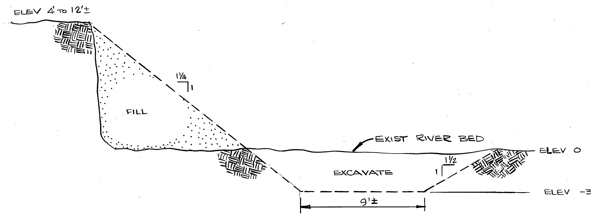
TYPICAL SECTION EARTHWORK SCALE 1" = 4'
