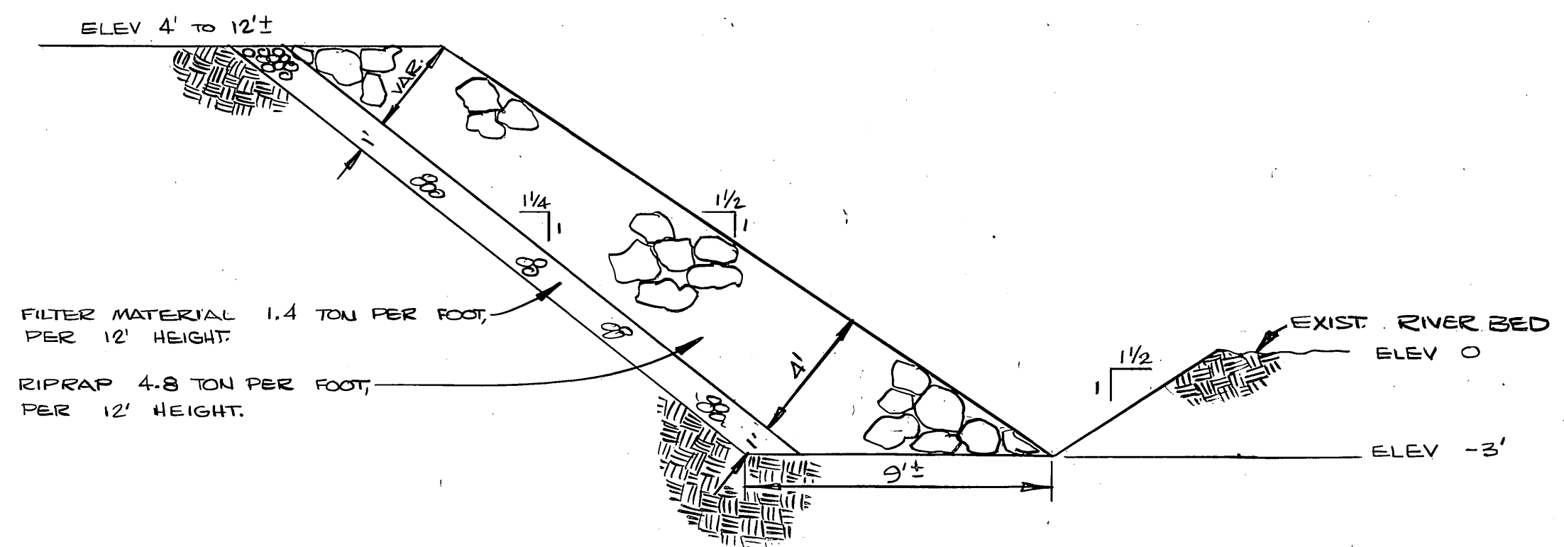
TYPICAL SECTION PROTECTION SCALE 1" = 4'
