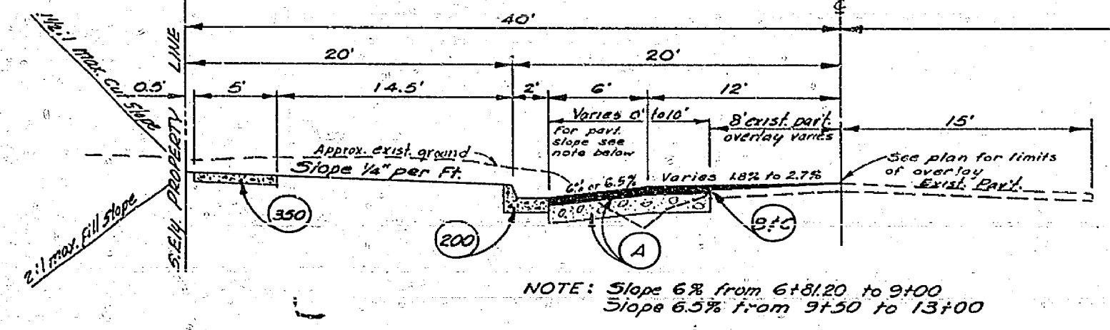
TYPICAL SECTION LINCOLN AVE. NO SCALE T.I. = 6
