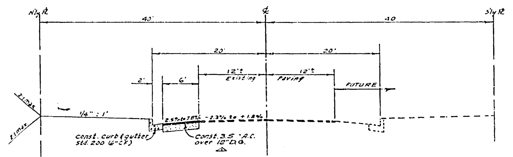
TYPICAL SECTION DOOLITTLE AVENUE NO SCALE 7.1. = 6
