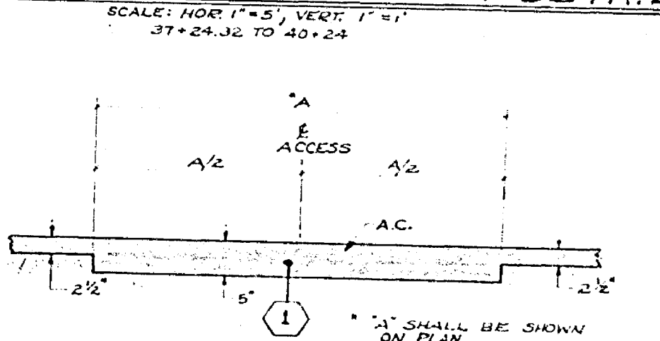
ACCESS DETAIL
