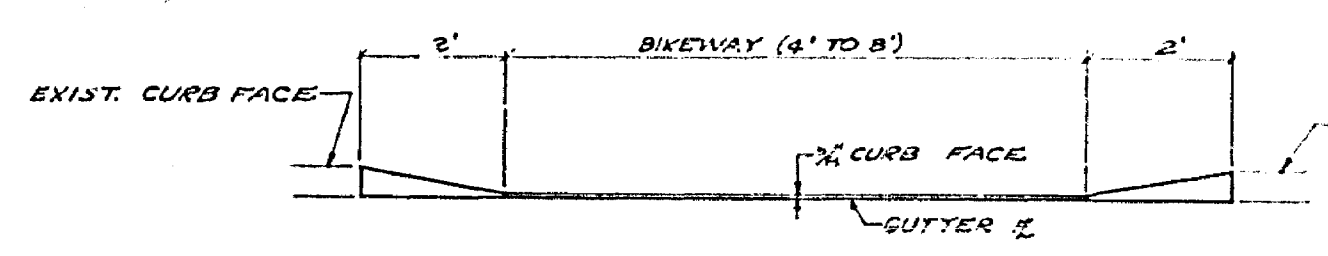
CURB DEPRESSION DETAIL
