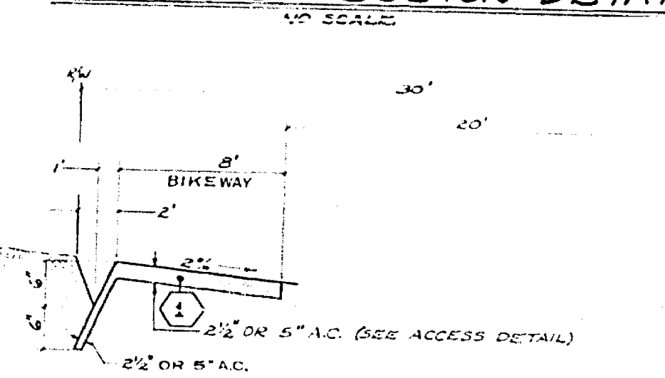
BIKEWAY PROTECTION DETAIL
