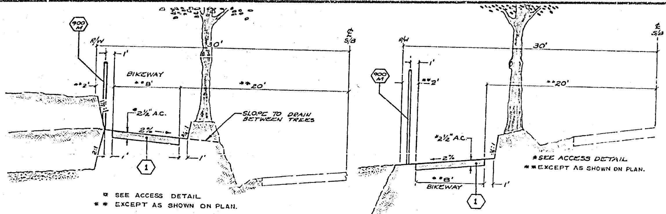
TYPICAL SECTION
