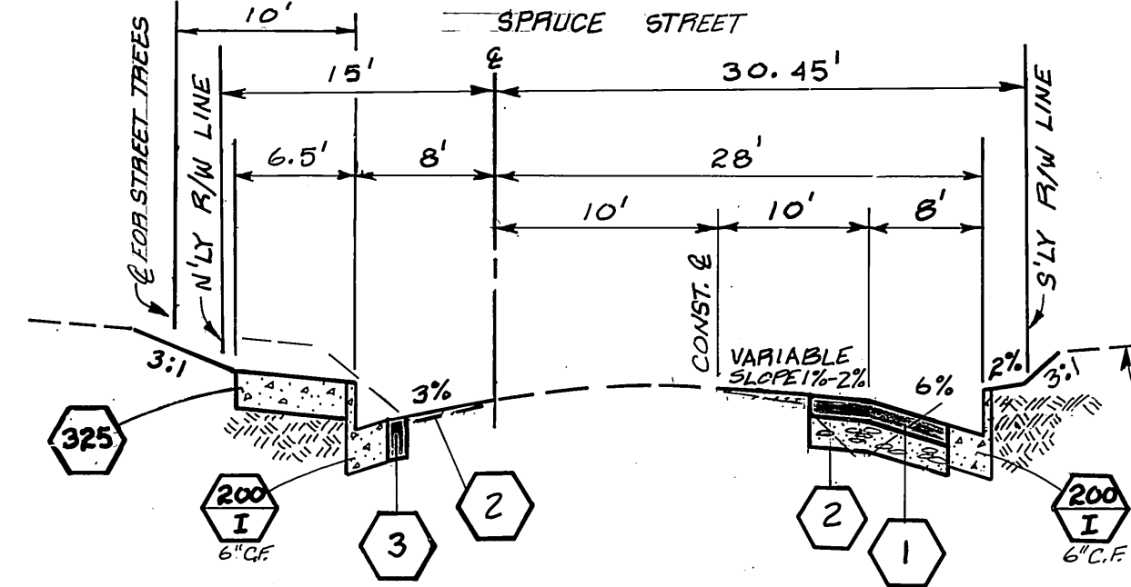
TYPICAL SECTION NO SCALE STD. 0+42.13 TO STD. 2+35
