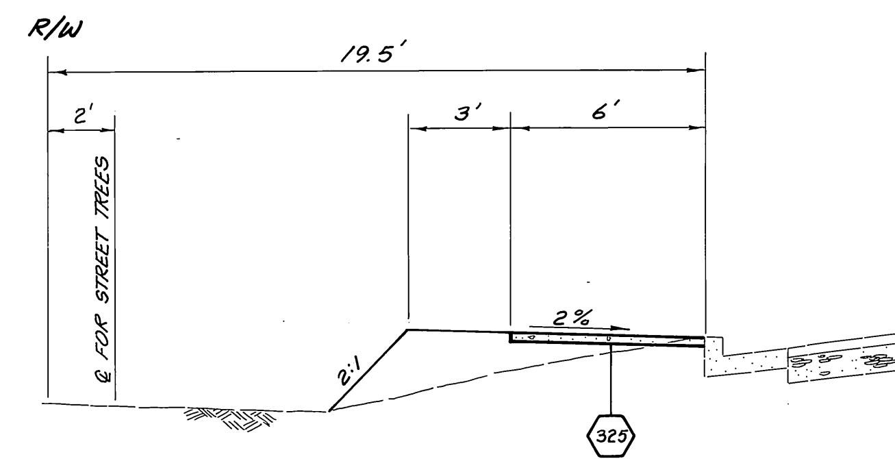
TYPICAL SECTION WARREN STREET TO MONTGOMERY STREET N.T.S.
