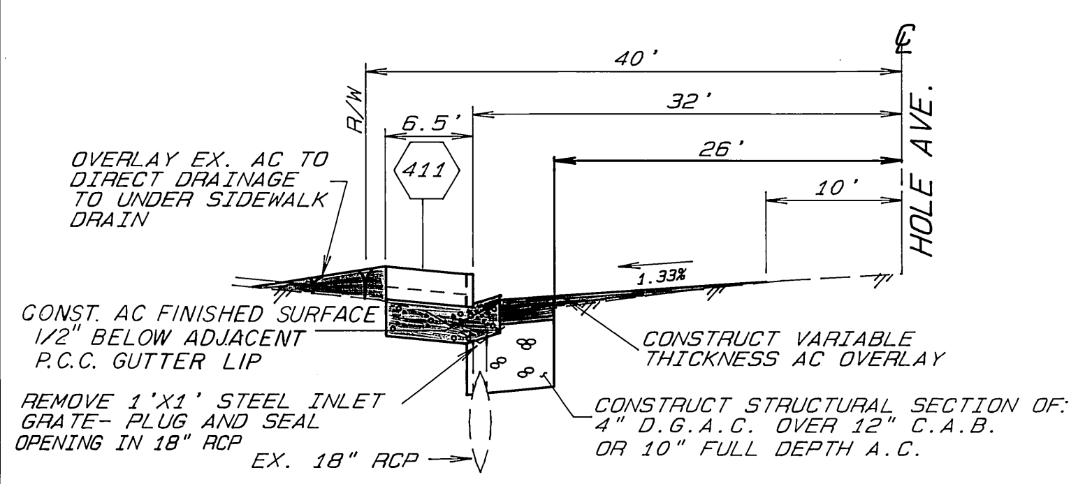
SECT. A-A UNDER SIDEWALK DRAIN DETAIL FOR PARKING LOT DRAINAGE SCALE: HORIZ. 1" = 10' VERT. 1" = 2'
