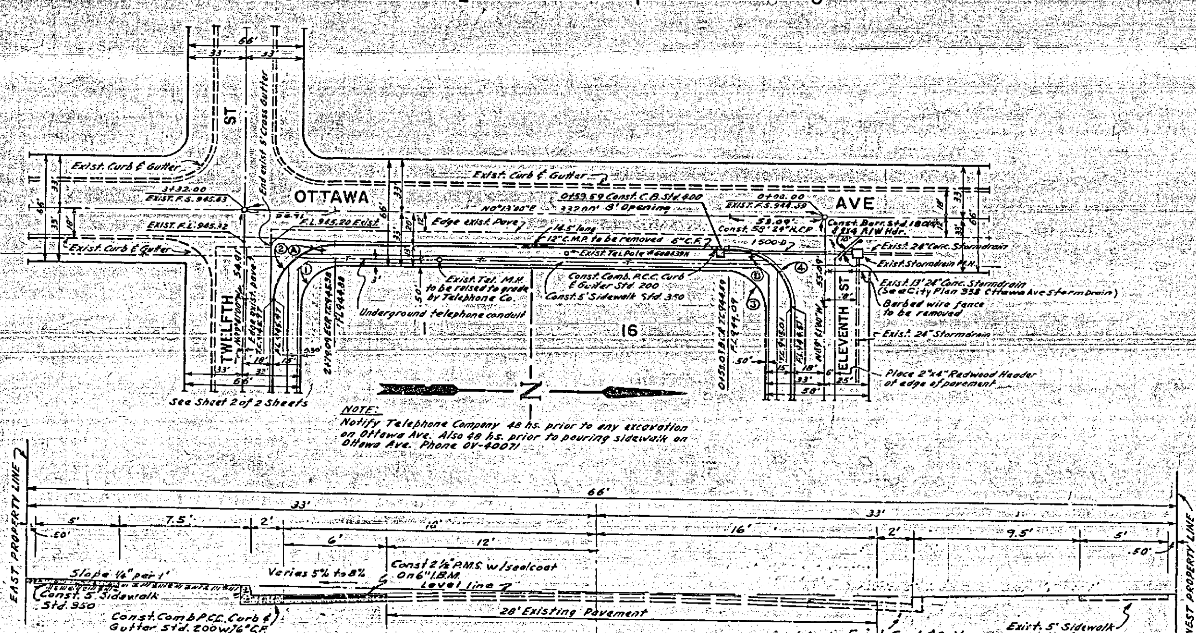
TYPICAL SECTION OF OTTAWA AVE SCALE 1"=5'
