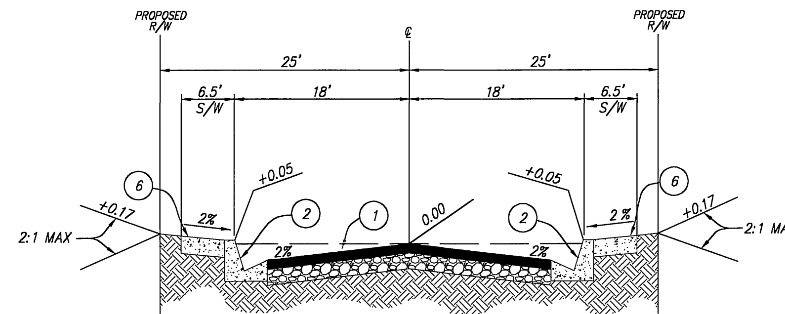
TYPICAL SECTION - TARA LANE NOT TO SCALE T.I. = 5.0
