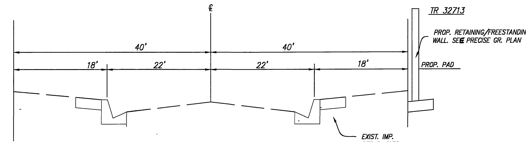
TYPICAL SECTION - MARY STREET NOT TO SCALE
