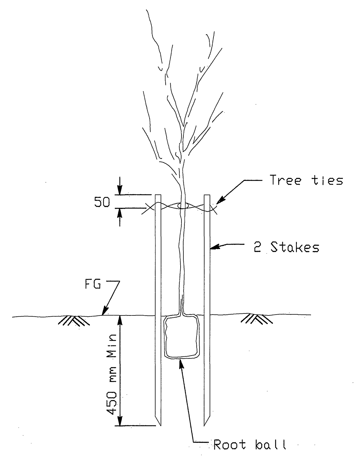
SECTION TREE STAKING
