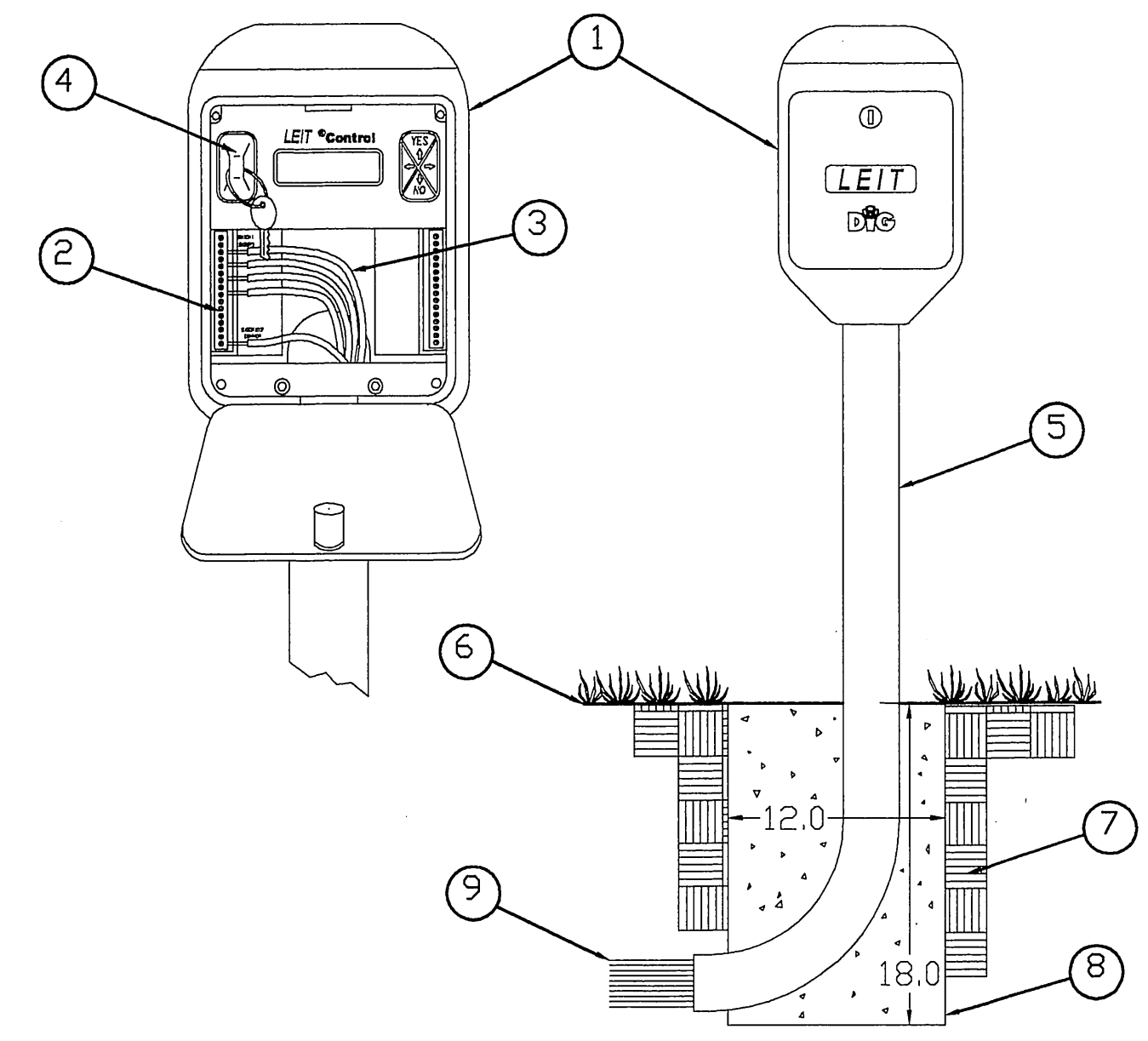
① LIGHT ENERGIZED IRRIGATION CONTROLLER LEIT CONTROL X , XR AND XRC
