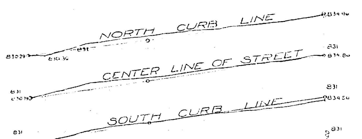
PROFILE OF BRISCOE ST. FROM MAGNOLIA AVE EASTERLY Scale - Horizontal 1 in. = 60 ft. Vertical 1 in. = 4 ft.
