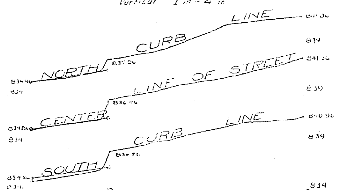
PROFILE OF BRISCOE ST. FROM MAGNOLIA AVE EASTERLY Scale - Horizontal 1 in. = 60 ft. Vertical 1 in. = 4 ft.
