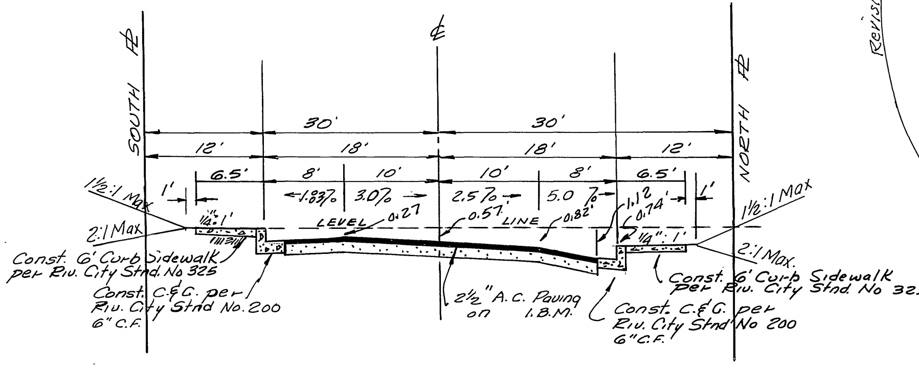
TYPICAL SECTION - OLD QUARRY RD. STA 1+63.36 SCALE - 1" = 10' - HOR 1" = 4' - VER
