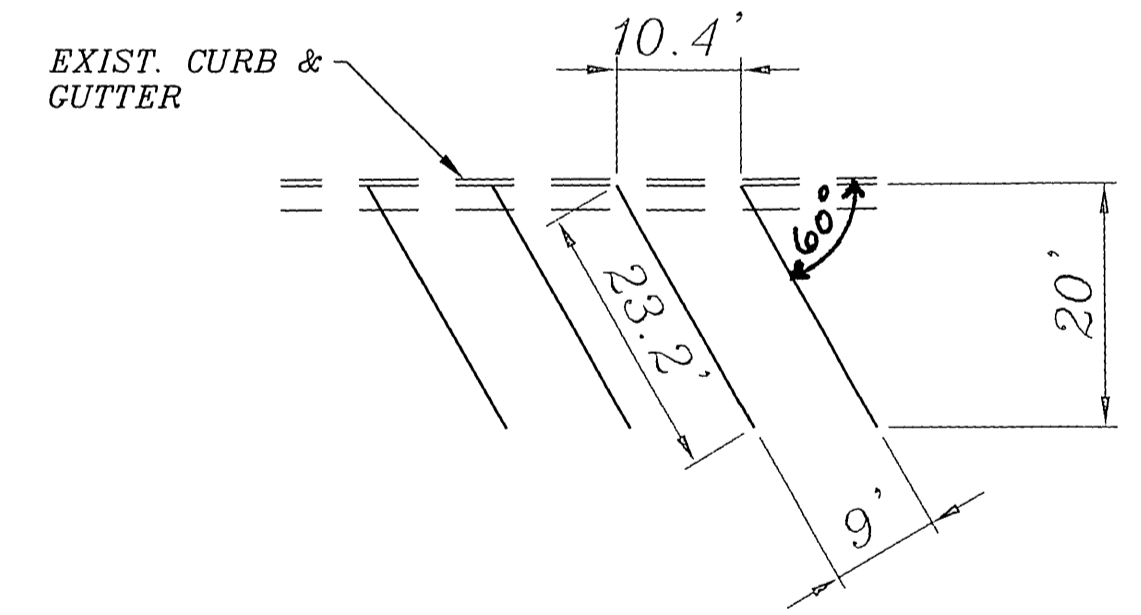
TYPICAL PARKING STALL DETAIL
