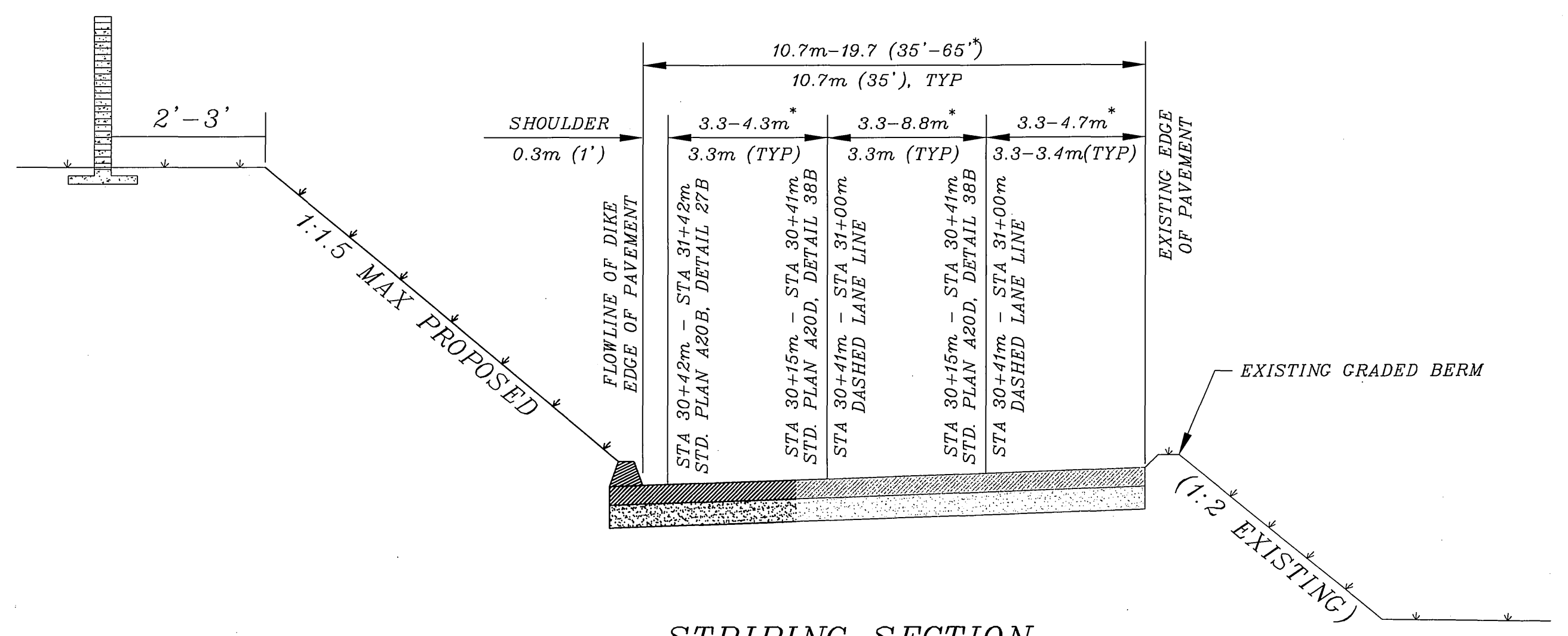
STRIPING SECTION NTS
