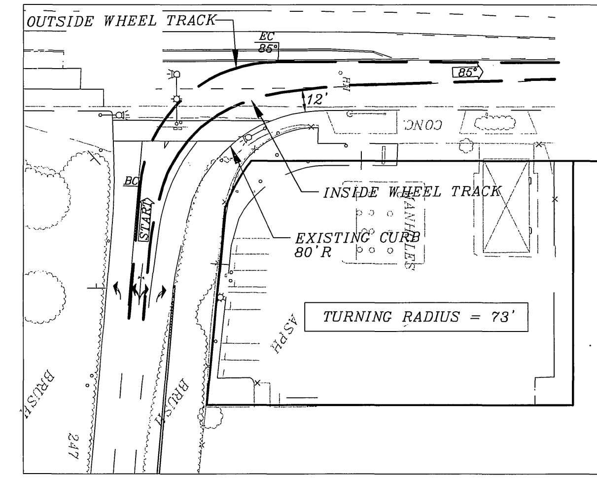
CALIFORNIA SEMI-TRAILER WHEEL TRACK DETAIL SCALE: NTS
