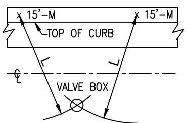
VALVE LOCATION TIES DETAIL (BY CITY FORCES)
